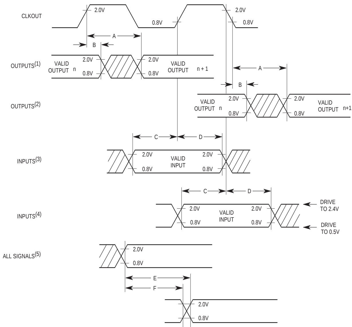
Figure 5. Drive Levels and Test Points For AC Specifications
