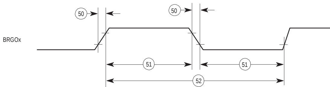
Figure 48. Baud Rate Generator Output Signals
