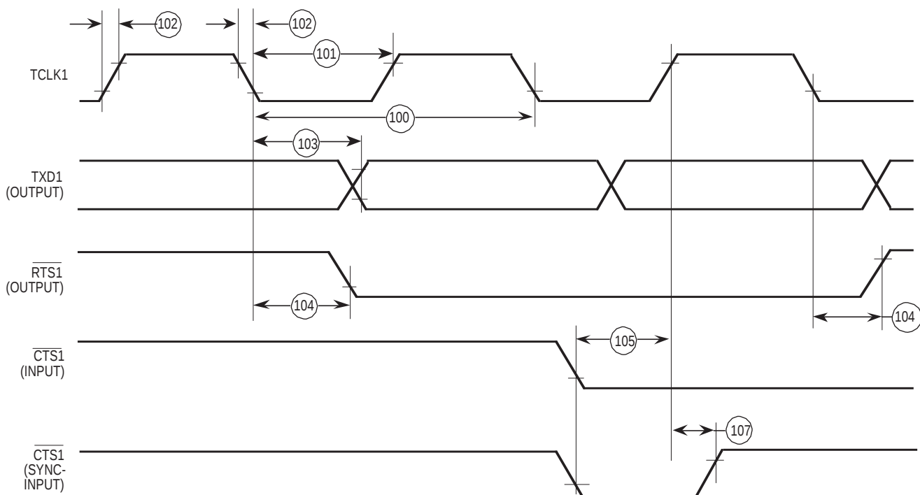
Figure 56. SCC NMSI Transmit
