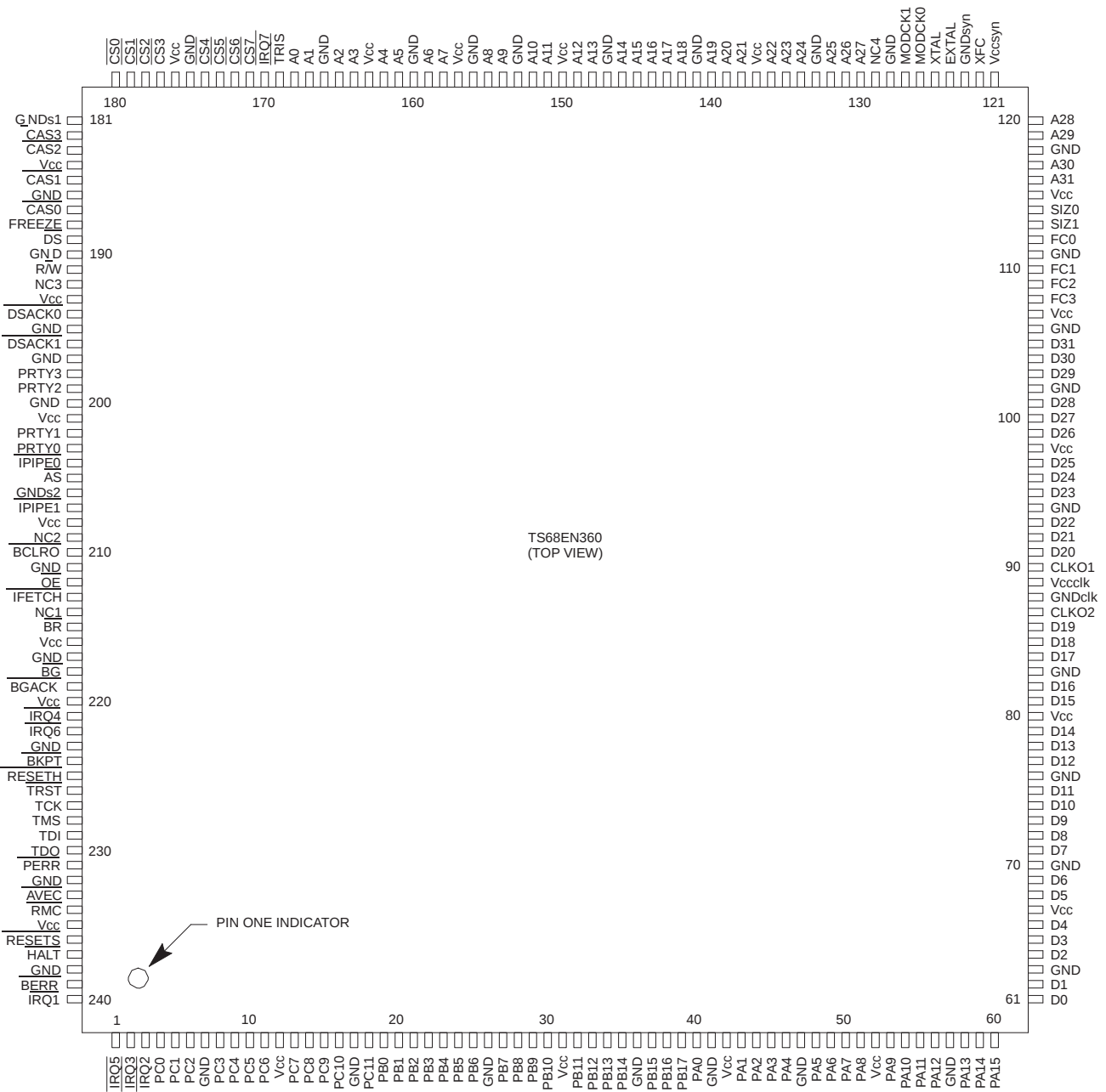
Figure 3. 240-lead Cerquad
