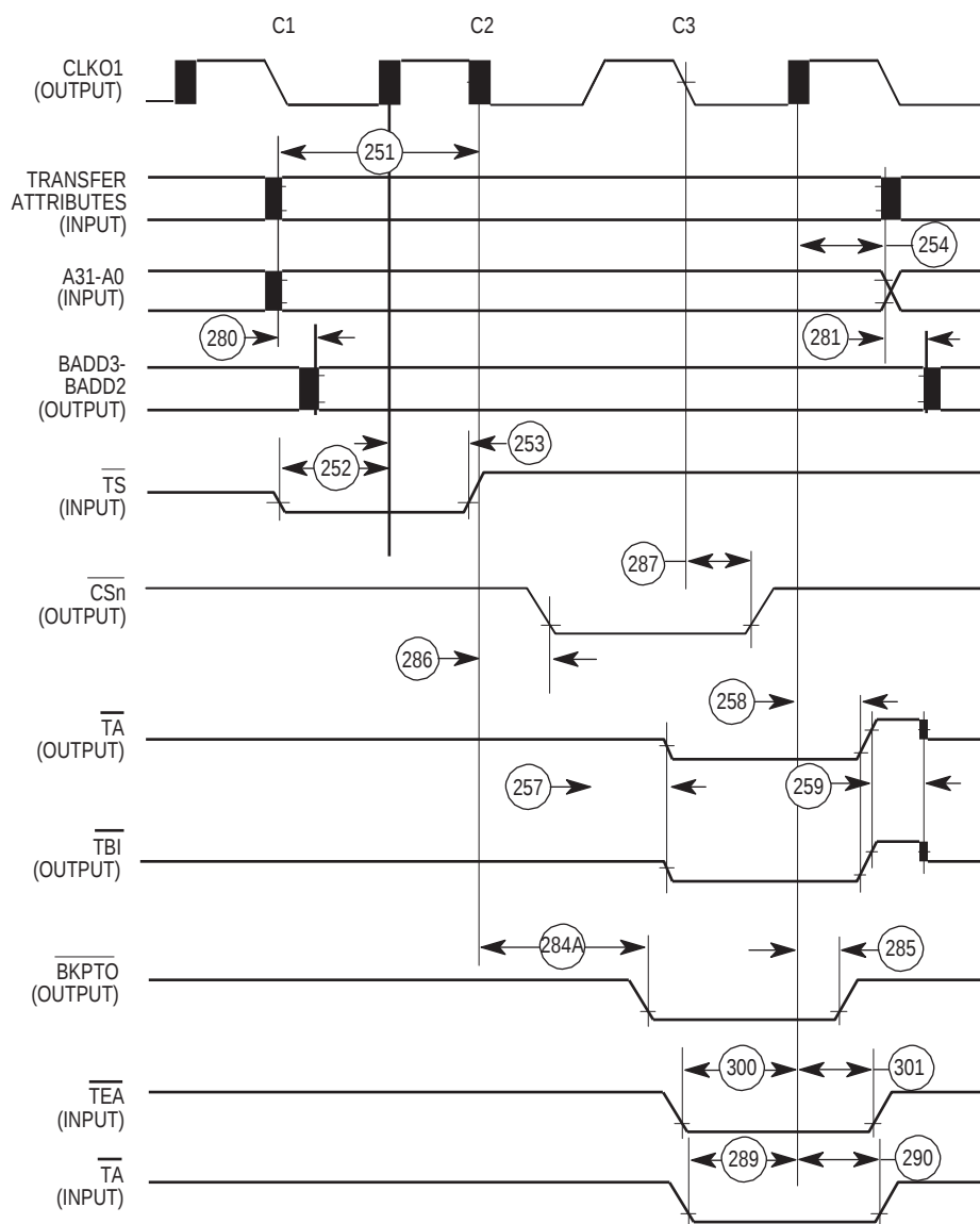
Figure 35. TS68040 SRAM Read/Write Cycles (TSS40 = 1, CSNT40 = 1)
